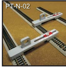
Adjustable Parallel Track Tool (N scale, metric/imperial)
